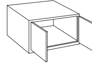
Wall Refrigerator Cabinet Width: 33", 36", 39" Depth: 24" Height: 12", 15", 18", 21", 24"
