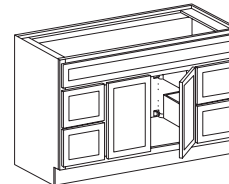
Vanity Sink Base with Drawers 1 Panel, 2 Doors and 4 Drawers VA482134D, VA602134D
