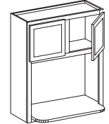
Wall Microwave Cabinet (WM) Width: 27" (Opening: 24" x 16")
